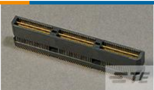
TE Part # 1-1658437-3 MSB0.80PL14ASY84DP,-,F,VCTY
