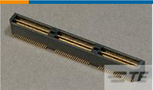
TE Part # 1-1658045-3 MSB0.80PL8ASY84DP,-,F,VCTY
