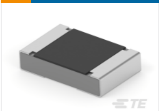
TE Part #8-2176482-2 RA73F 2A 357R 0.1% 5K RL
