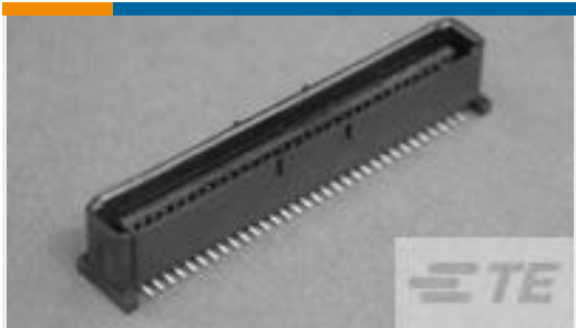
TE Part #5146897-1 1FHP,64,30A/S,S,C,S08
