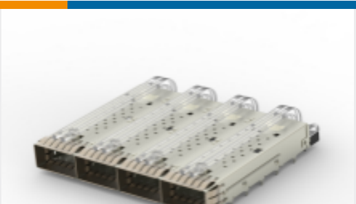
TE Part #2170746-1 CAGE ASSY, 1X4, QSFP28, SPRING, LP
