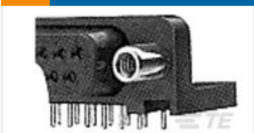
TE Part #5788797-1 09 HTMSFL ASSY RA 318 (SL,BL)
