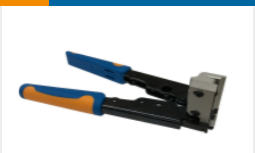
TE Part #2305570-1 Strip Terminal Cutter-Side Feed-No Crimp
