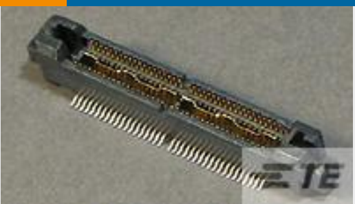
TE Part # 5767025-2 MICTOR .707 PLUG ASSY, 76 POS.
