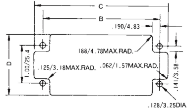
Layout for Back Chassis Mounting
