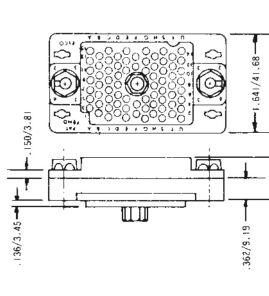
Receptacle with Fixed Nut 007
