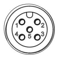
Conn. 1 & 2 & 3 & 4 & 5 Pin Assignments Front View
