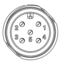
Conn. 6 Pin Assignments Front View
