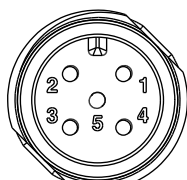
Conn.3 Pin Assignments Front View
