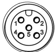
Conn.1&2 Pin Assignments Front View
