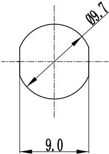
Mounting Hole
