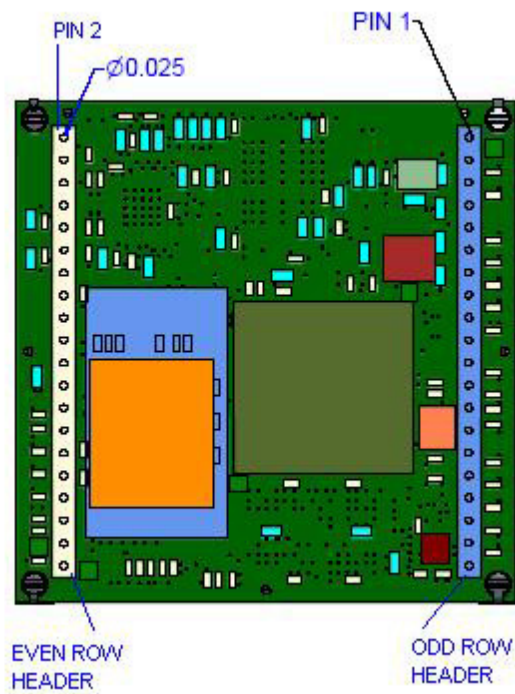
Figure 2-11. Bottom View
