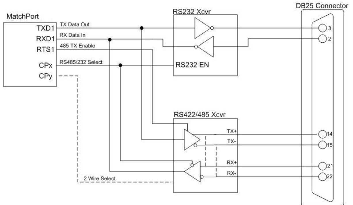
Figure 2-6. Separate RS232/422 Transceivers
