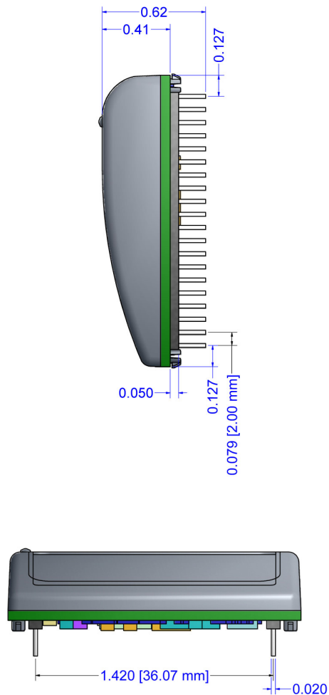
Figure 2-9. Side Views
