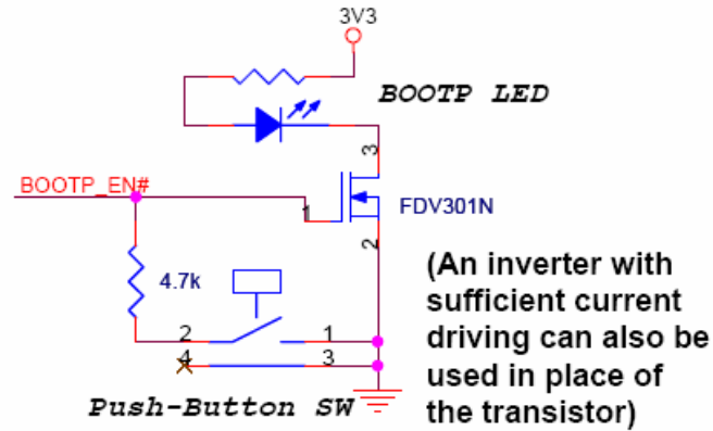
BOOTP_EN# application circuit
