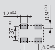
pad layout
