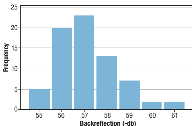
3M™ Lapping Film 865X Backreflection Results
