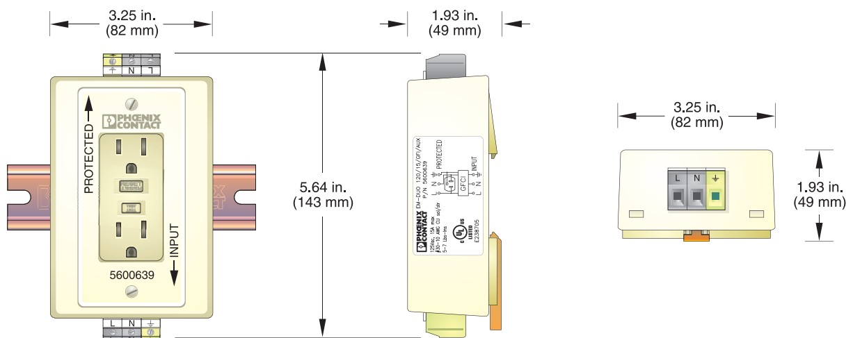
Figure 2 EM-DUO-120/.../AUX... dimensions
