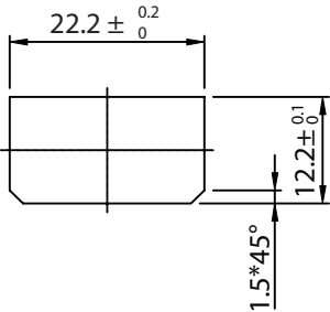
PANEL CUTOUT Panel Thickness Range: 1.0mm ~ 1.8mm
