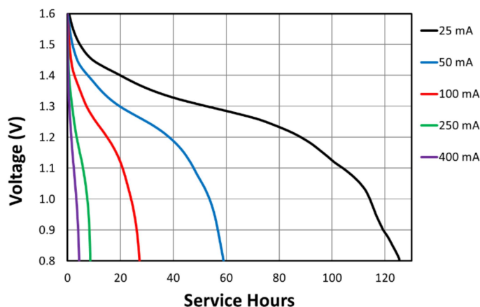
Constant Current
