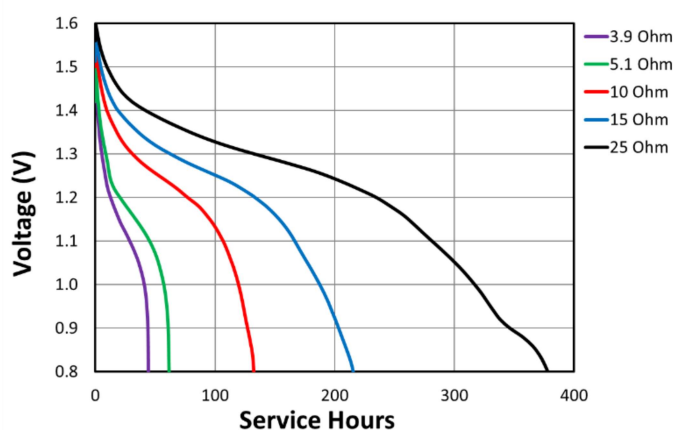
Constant Resistance
