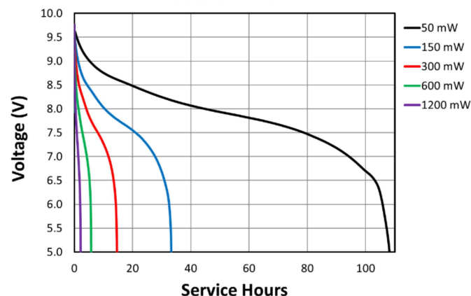
Constant Power
