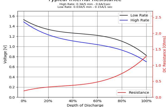
Typical Internal Resistance
