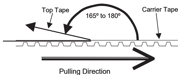
Fig.9 Peeling Strength
