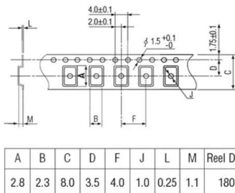
Figure 3) Pocket Tape Dimensions
